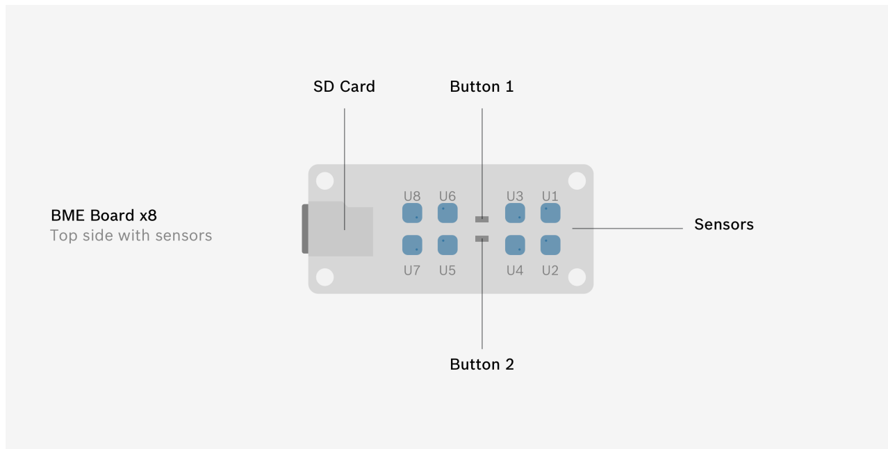
Fig. 4: BME688 Board
