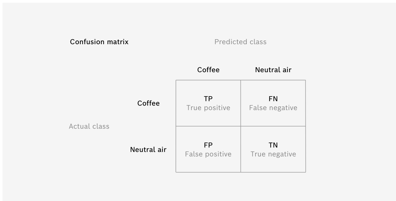
Fig. 17: Confusion Matrix
