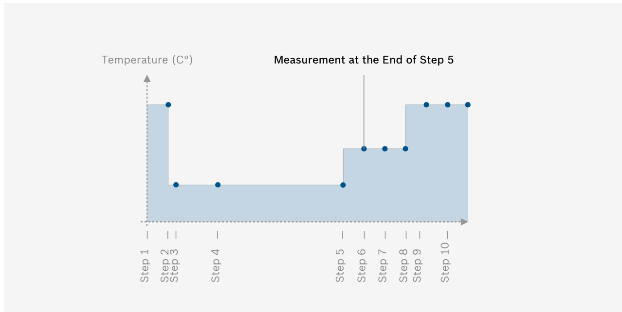
Fig. 5: Heater Profile
